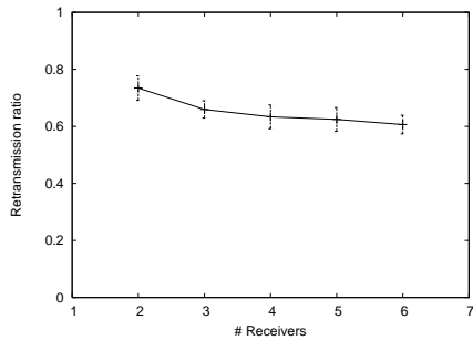
Figure 18: Unicast experiment results under a varying number of clients.
